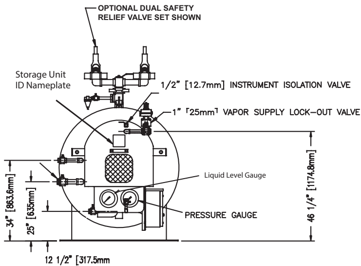
Figure 1: 2 3/4 Ton Tank
