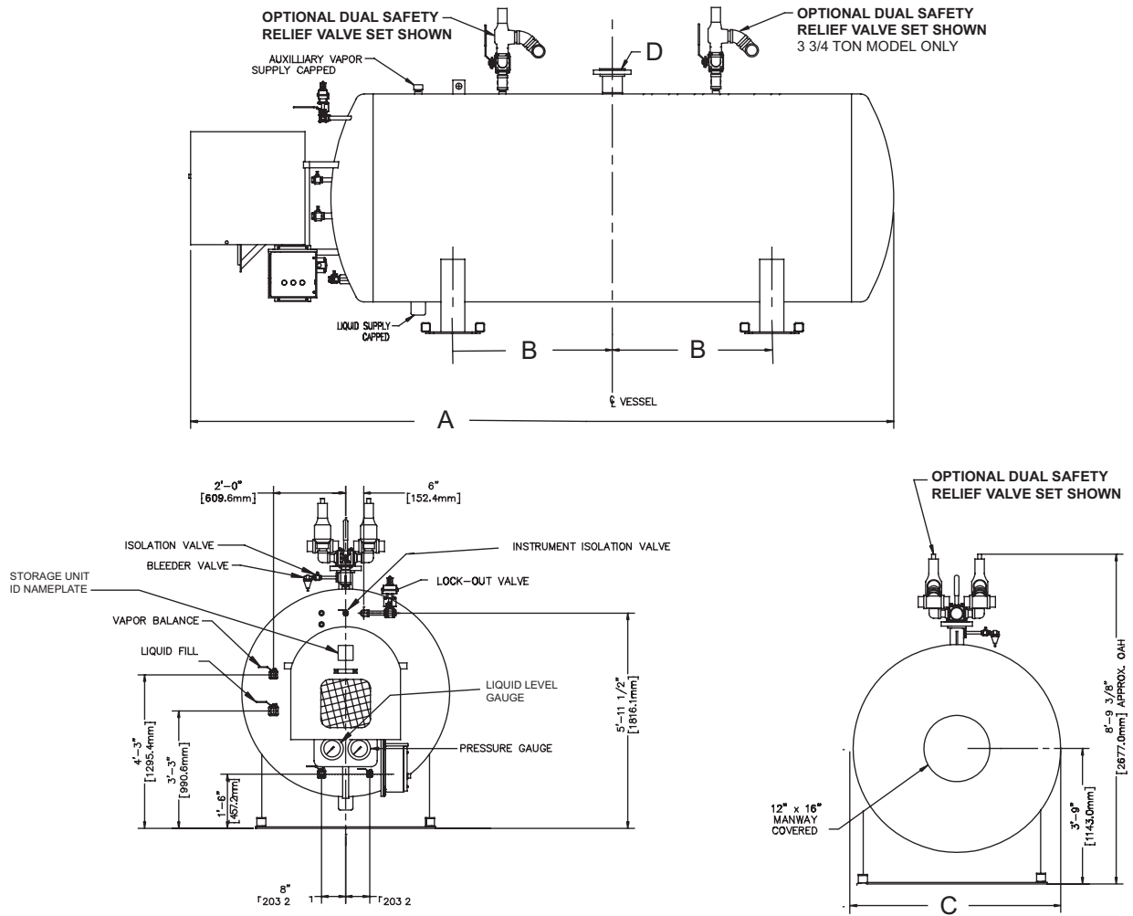
Figure 2: 3 3/4 through 12 Ton Tanks
