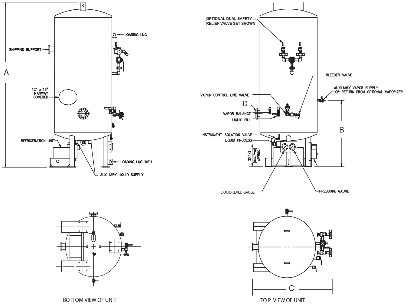
Figure 7: 6 Ton Tank
