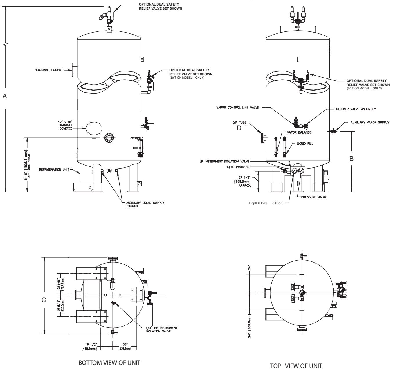
Figure 8: 14, 26, and 30 Ton Tanks
