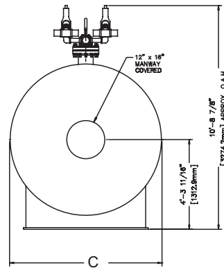
Figure 6: 30 through 60 Ton Tanks
