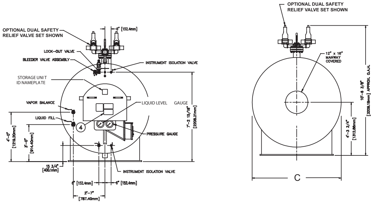
Figure 5: 26 Ton Tank
