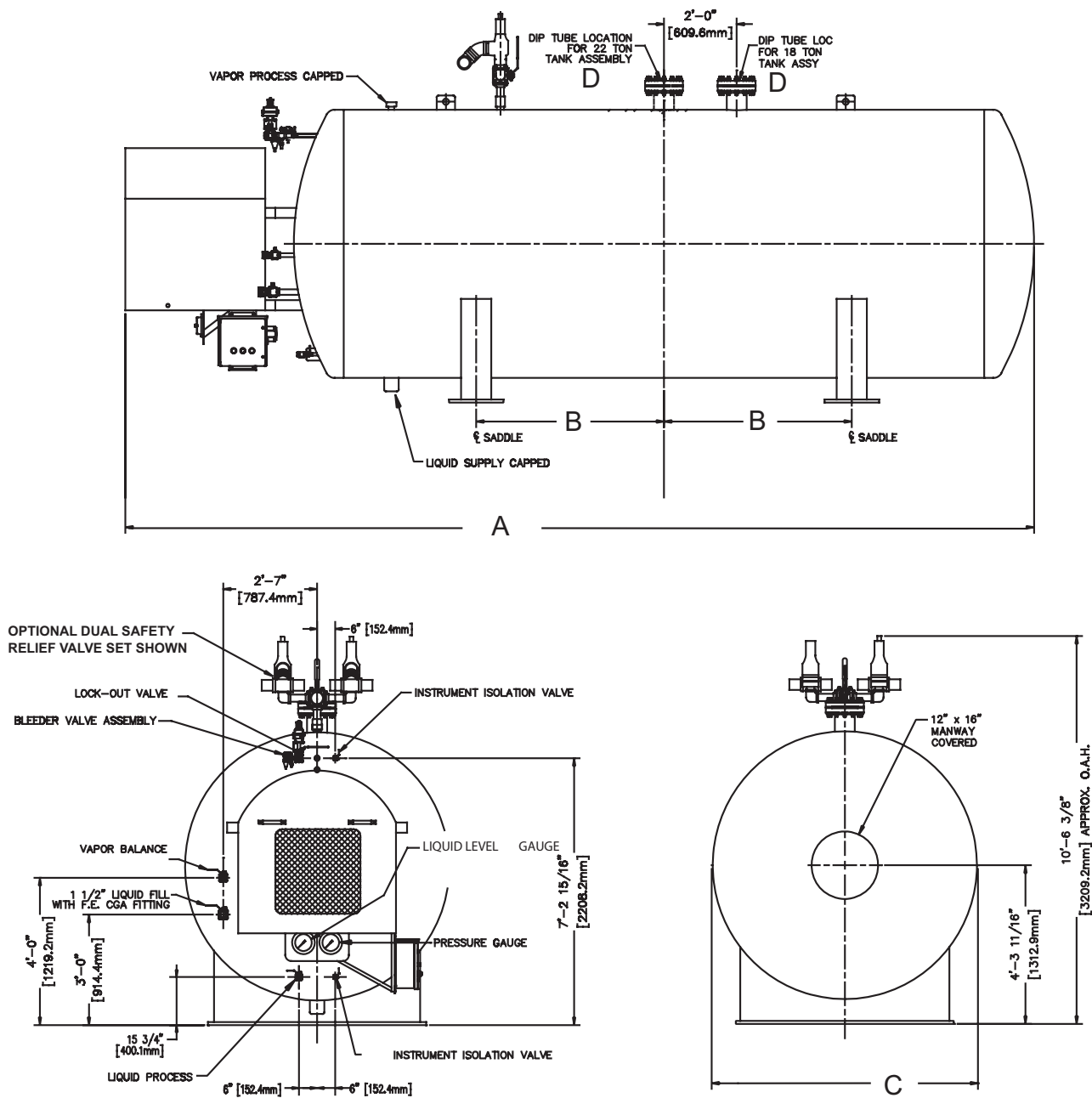
Figure 4: 18 and 22 Ton Tanks
